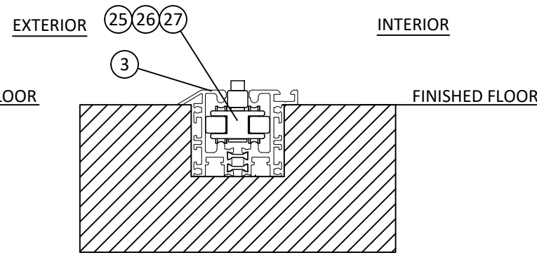
FLUSH THRESHOLD (SEE INSTALLATION DETAILS X/11 & Y/11 ABOVE)
