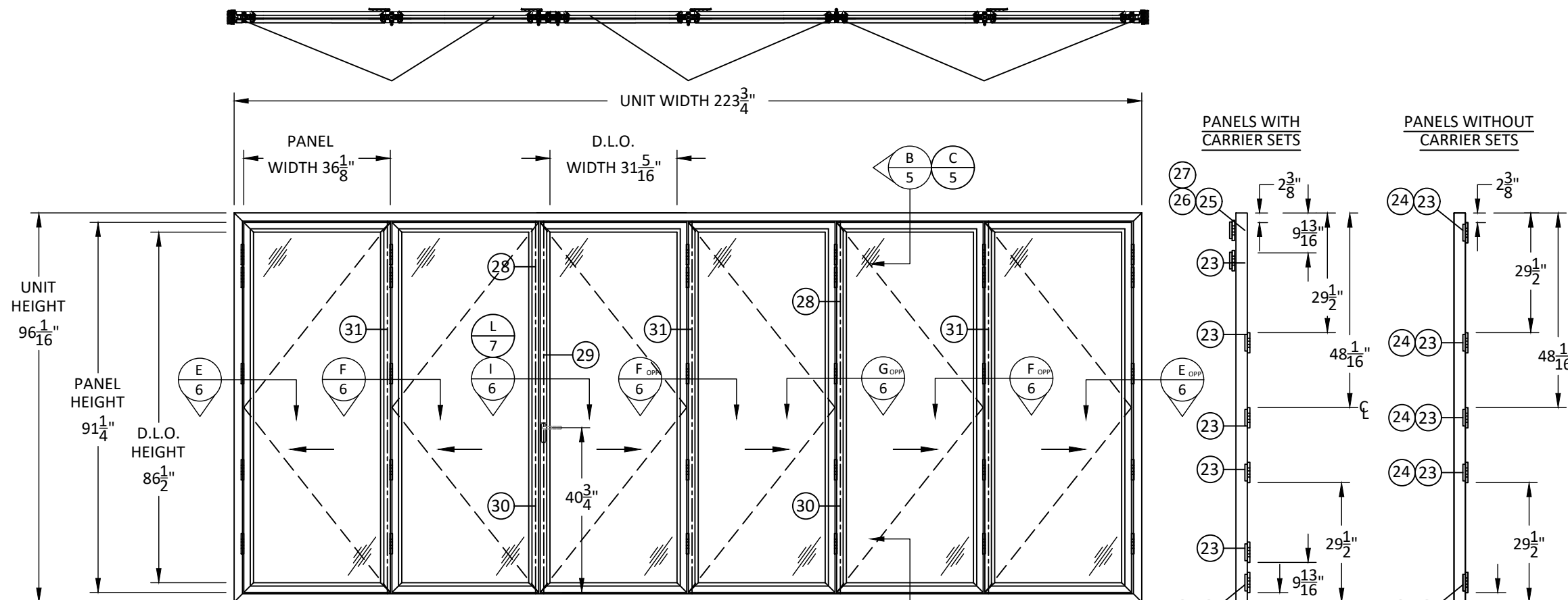
ELEVATION INSWING 2L4R UNIT SHOWN
