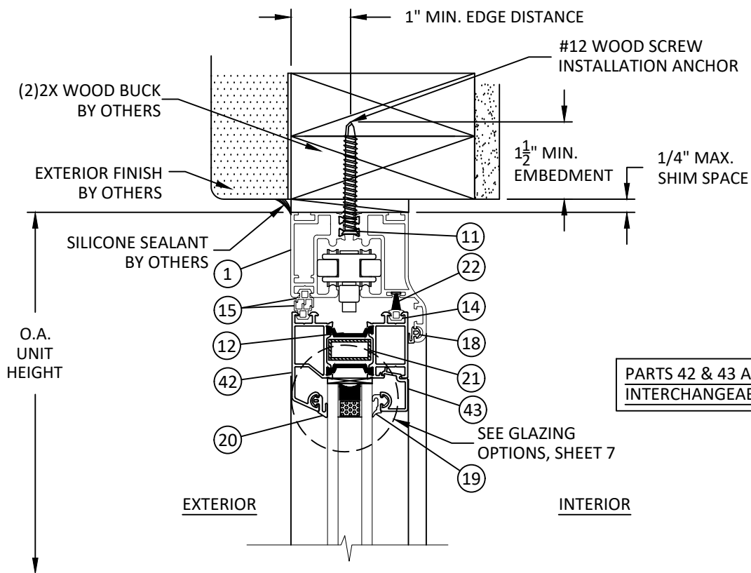
B 5 VERTICAL SECTION HEAD - 2X WOOD BUCK
