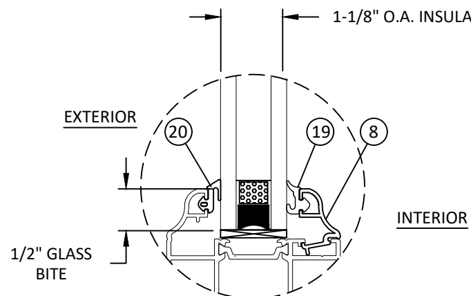
GLAZING DETAIL 1
