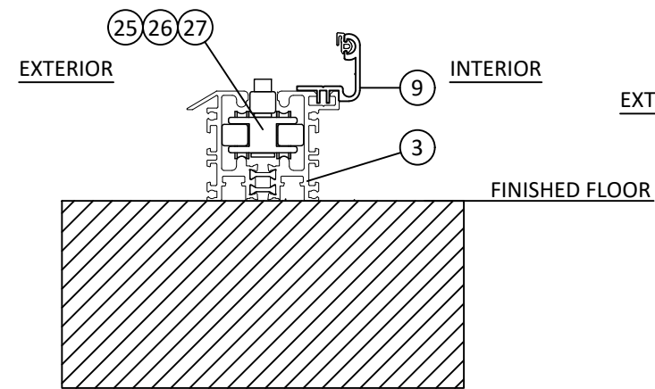
WATER BARRIER THRESHOLD (SEE INSTALLATION DETAIL A/5)
