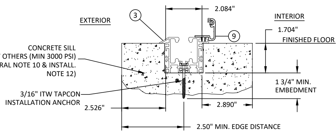
Y 12 RECESSED U-CHANNEL CONCRETE INSTALLATION PREPARATION
