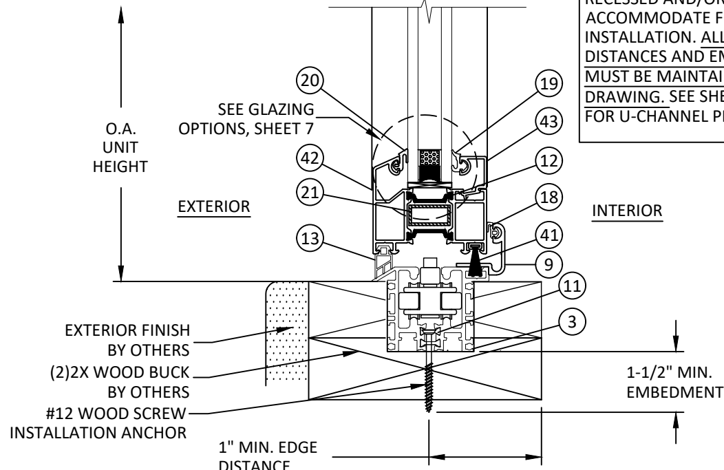
D 5 VERTICAL SECTION RECESSED U-CANNEL - 2X WOOD FRAME FLUSH THRESHOLD
